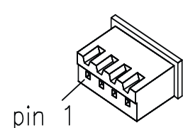
JST XHP-4 "CONN 3"
