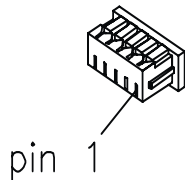
Molex 51021-0500 "CONN 1"
